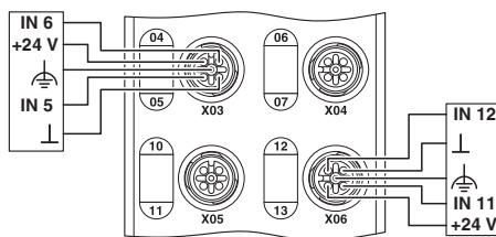
Connection diagram
